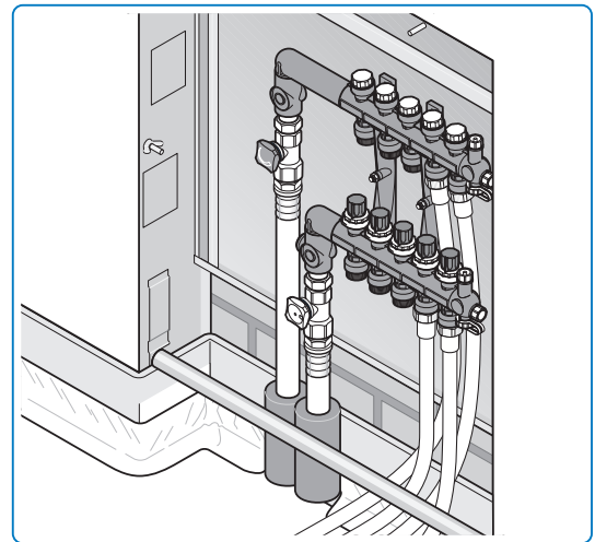
Connection of the PE-Xa 9.9 system pipes or PE-Xa 20 zone supply lines to the plastic Uponor manifold
