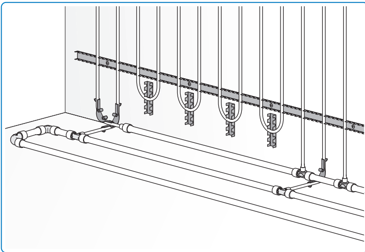
Connection of the PE-Xa 9.9 system pipes to a PE-Xa Tichelmann ring using Q&E connectors.
